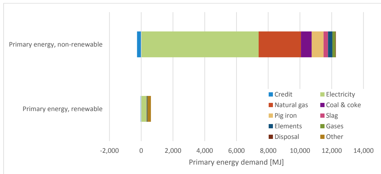
Figure 4-2: Primary energy demand breakdown
