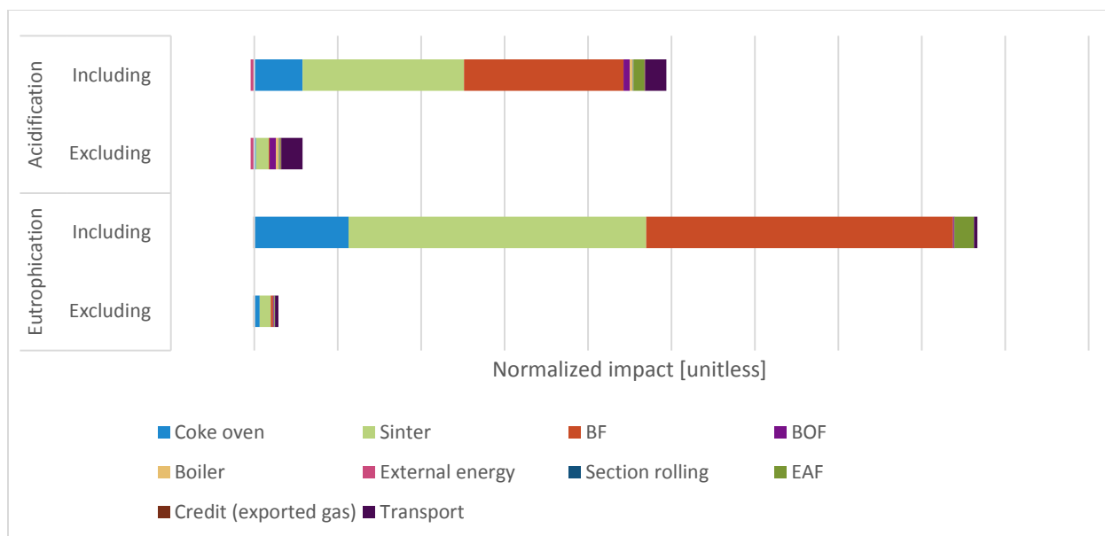
Figure 4-6: Normalized structural sections results including and excluding ammonia emissions to water
